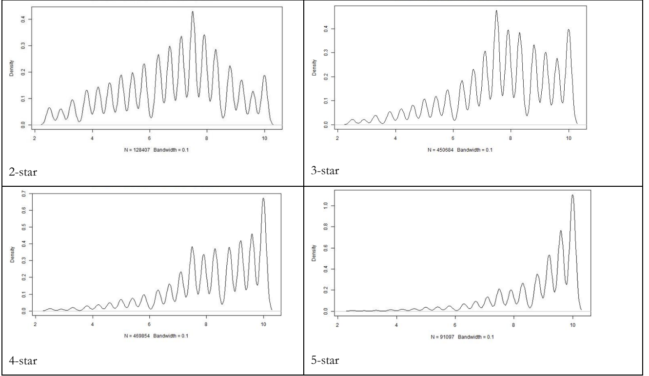
Fig. 4. Kernel density distributions
